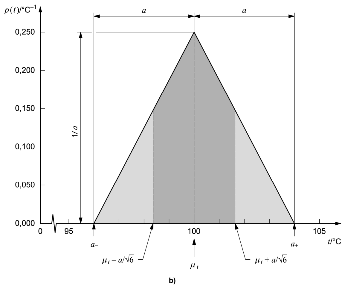
Figure 2 — Graphical illustration of evaluating the standard uncertainty of an input quantity from an a priori distribution
